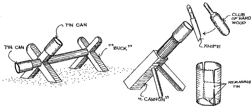
Fig. 23: Devices for the preparation of tin cans
