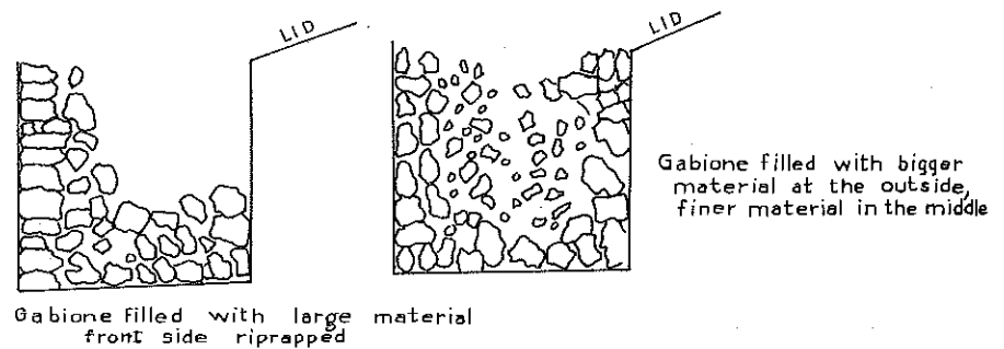
Fig. 10: Filling of a gabion
