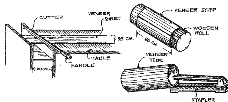
Fig. 24: Manufacture of veneer pots
