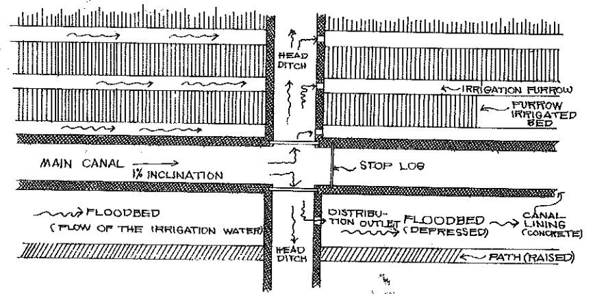
Fig. 4: Layout of flood irrigation
