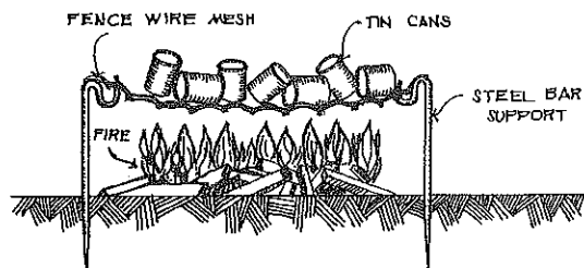
Fig. 22: Sterilization of tin cans
