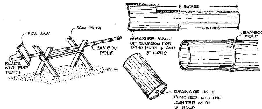
Fig. 21: Preparation of boho pots
