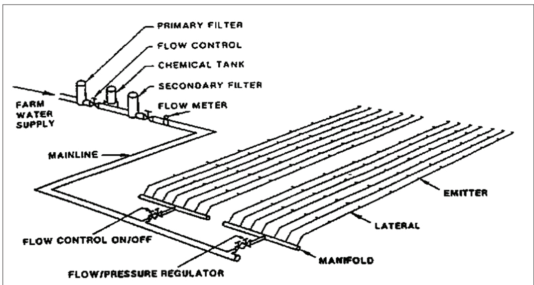
Fig.12. Basic components of a drip irrigation system Source: FAO, Irrigation and Drainage Paper. Rome, 1984)
