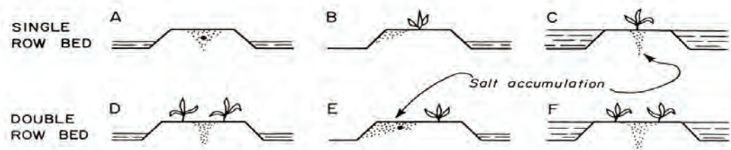
Fig. 20. Flat top beds and irrigation practices (source: Water quality for agriculture)
